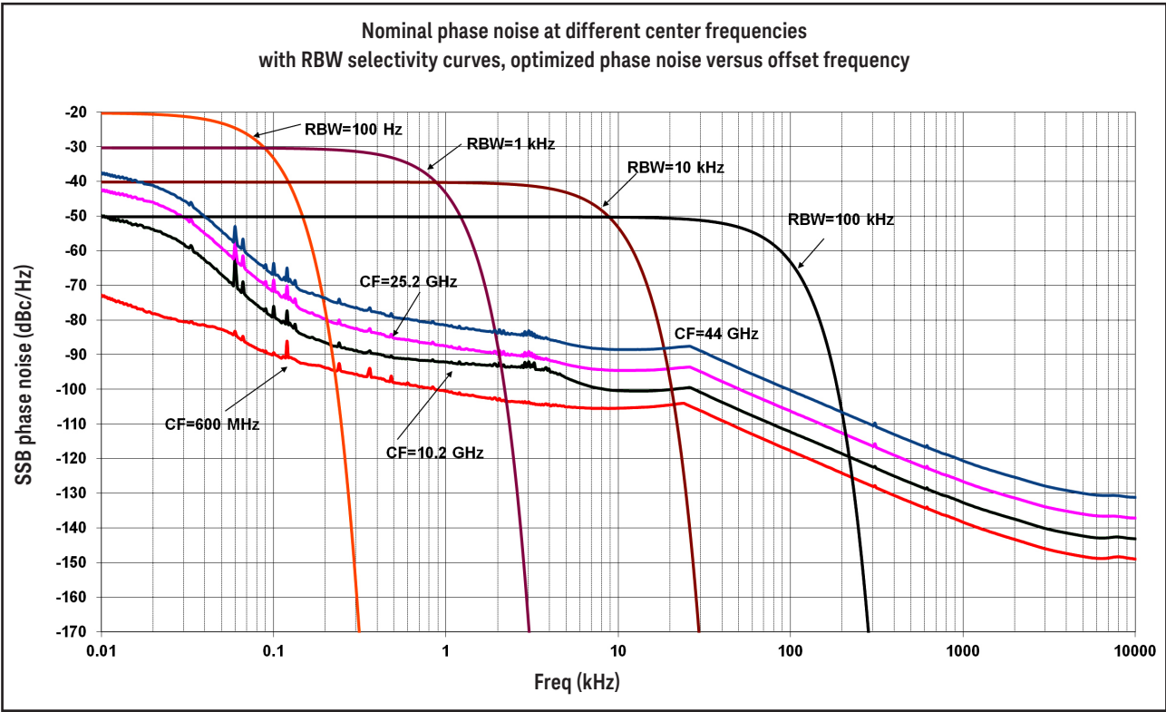
Figure 3. Nominal phase noise at different center frequencies with SN prefix ≥ MY/SG/US5648 that ships standard with N9010A-EP5.
